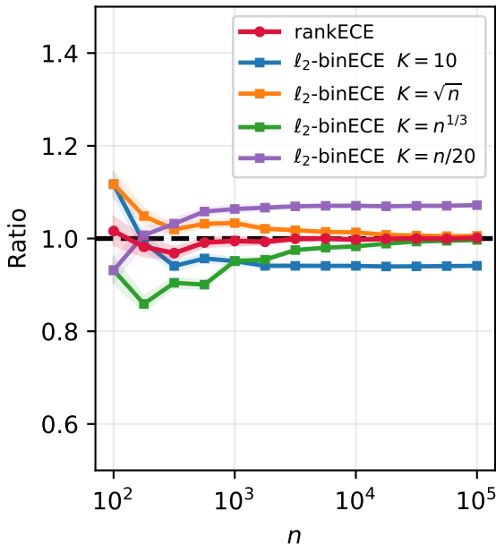
Random Fourier
